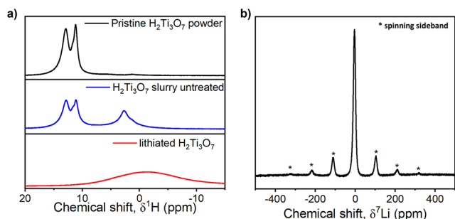
Figure 8. Ex situ solid-state NMR of \text{H}_2\text{Ti}_3\text{O}_7 before and after \text{Li}^+ insertion. (a) Solid-state ^1\text{H} NMR of pristine \text{H}_2\text{Ti}_3\text{O}_7 powder (black), \text{H}_2\text{Ti}_3\text{O}_7 dried slurry (blue), and \text{H}_2\text{Ti}_3\text{O}_7 after 10 cycles and holding at 1 V vs \text{Li}/\text{Li}^+ for 24 h in 1 M \text{LiClO}_4 in PC. (b) Solid-state ^7\text{Li} NMR of \text{H}_2\text{Ti}_3\text{O}_7 after 10 cycles and holding at 1 V vs \text{Li}/\text{Li}^+ for 24 h in 1 M \text{LiClO}_4 in PC.
