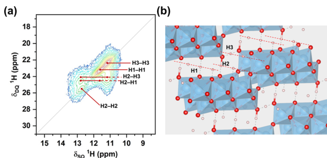
Figure 9. (a) \text{T}^1\text{H}\text{--}^1\text{H} DQ/SQ correlation NMR spectroscopy for pristine 3s-HTO powder. (b) DFT calculated structure of 3s-HTO. Red dashed line represents the b -axis alignment of hydrogen atoms.
