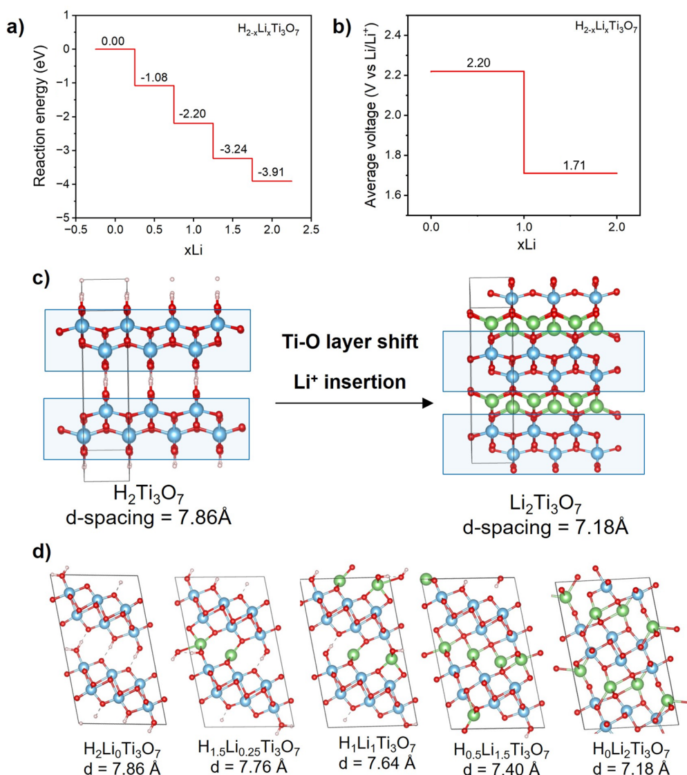
Figure 6. (a) DFT-computed reaction energy of \text{H}_2\text{Ti}_3\text{O}_7 + x\text{Li} (\text{s}) \rightarrow \text{H}_{2-x}\text{Li}_x\text{Ti}_3\text{O}_7 + 1/2 x\text{H}_2 (\text{g}) for x from 0 to 2. (b) Voltage profile for first/second half lithiation step. (c) DFT-calculated structures of \text{H}_2\text{Ti}_3\text{O}_7 and \text{Li}_2\text{Ti}_3\text{O}_7 showing a shift in the Ti–O layer to accommodate full \text{Li}^+ insertion. (d) Models for partially lithiated titanate from \text{H}_2\text{Li}_0\text{Ti}_3\text{O}_7 to \text{H}_0\text{Li}_2\text{Ti}_3\text{O}_7 (Ti: blue; Li: green; H: white; O: red).
